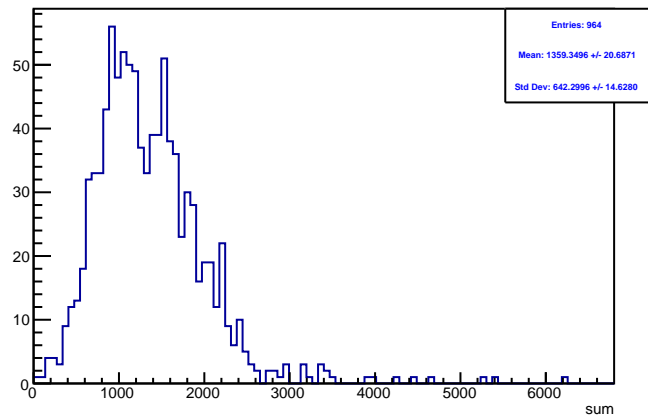
Run 4595 triggerwise, sums: Beam OFF
