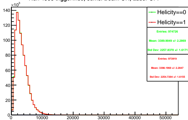
Run 4595 triggerwise, sums: Beam ON, Laser OFF
