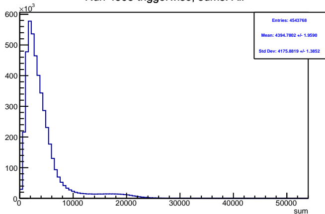
Run 4595 triggerwise, sums: All
