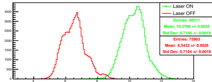
Run 4596 quartetwise, negH0: Beam ON
