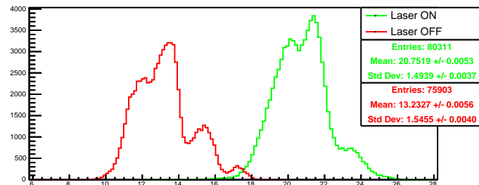
Run 4596 quartetwise, summ0: Beam ON
