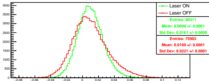
Run 4596 quartetwise, asym0: Beam ON
