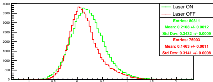
Run 4596 quartetwise, diff0: Beam ON
