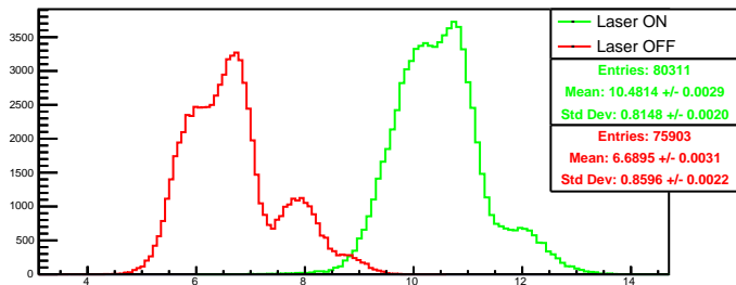
Run 4596 quartetwise, posH0: Beam ON
