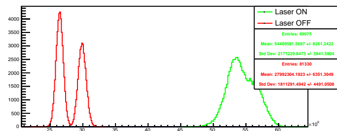
Run 4597 quartetwise, summ4: Beam ON
