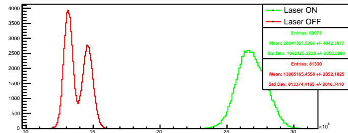
Run 4597 quartetwise, negH4: Beam ON
