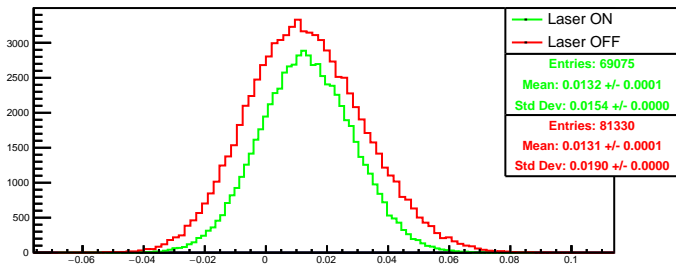
Run 4597 quartetwise, asym4: Beam ON
