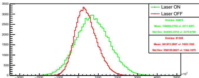
Run 4597 quartetwise, diff4: Beam ON
