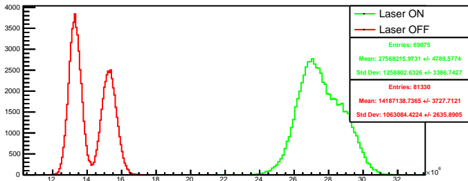
Run 4597 quartetwise, posH4: Beam ON
