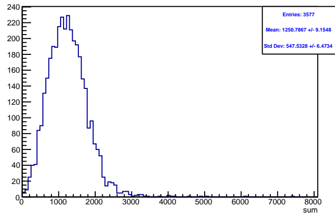
Run 4597 triggerwise, sums: Beam OFF
