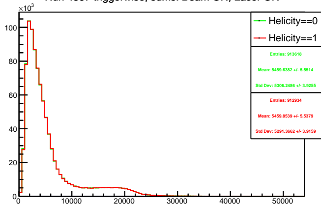
Run 4597 triggerwise, sums: Beam ON, Laser ON
