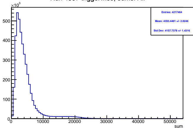
Run 4597 triggerwise, sums: All
