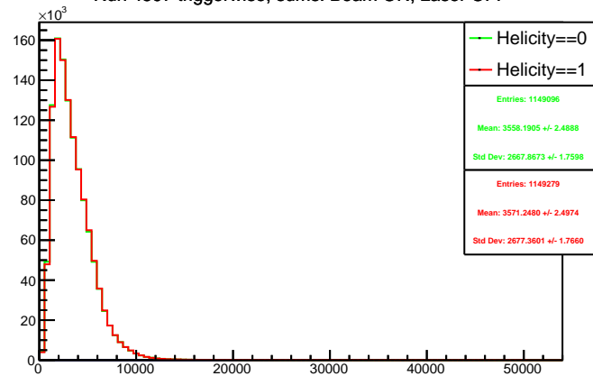
Run 4597 triggerwise, sums: Beam ON, Laser OFF
