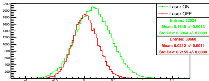
Run 4600 quartetwise, diff0: Beam ON
