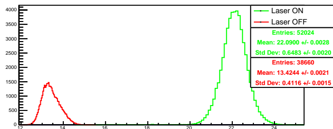
Run 4600 quartetwise, summ0: Beam ON
