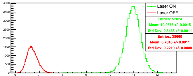
Run 4600 quartetwise, negH0: Beam ON
