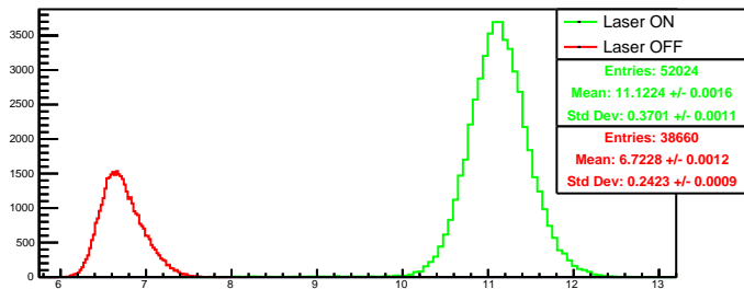
Run 4600 quartetwise, posH0: Beam ON
