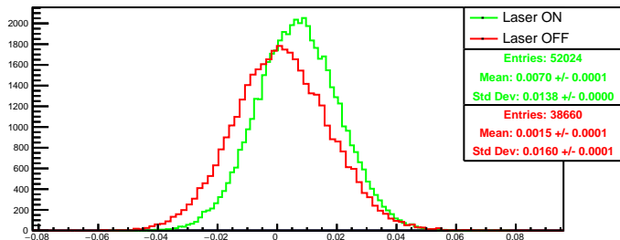
Run 4600 quartetwise, asym0: Beam ON
