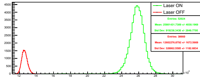
Run 4600 quartetwise, negH4: Beam ON
