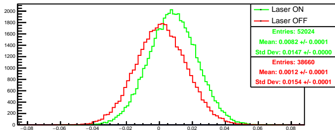
Run 4600 quartetwise, asym4: Beam ON
