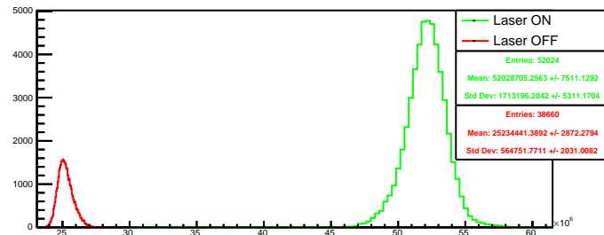
Run 4600 quartetwise, summ4: Beam ON
