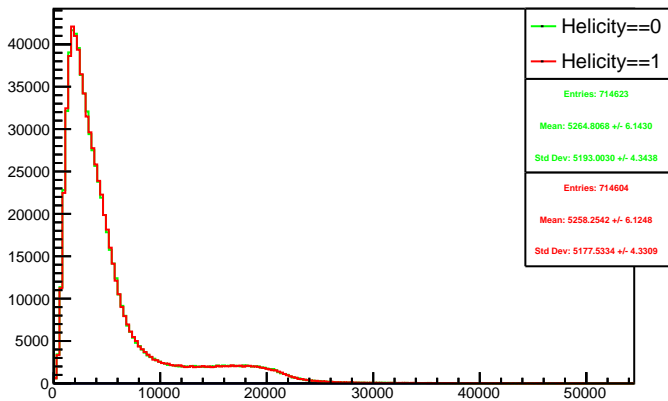
Run 4600 triggerwise, sums: Beam ON, Laser ON
