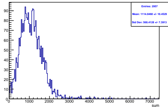
Run 4600 triggerwise, sums: Beam ON, Laser OFF
