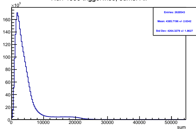
Run 4600 triggerwise, sums: All
