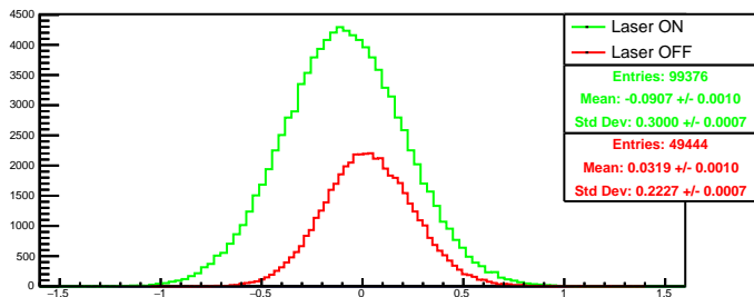
Run 4601 quartetwise, diff0: Beam ON
