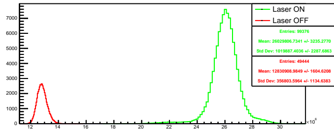
Run 4601 quartetwise, negH4: Beam ON
