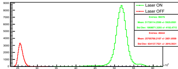
Run 4601 quartetwise, summ4: Beam ON
