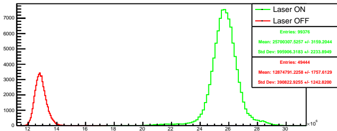
Run 4601 quartetwise, posH4: Beam ON
