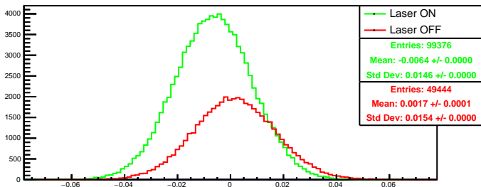
Run 4601 quartetwise, asym4: Beam ON
