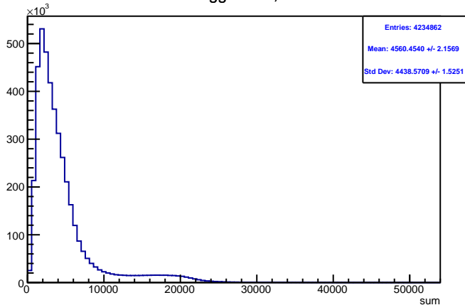
Run 4601 triggerwise, sums: All
