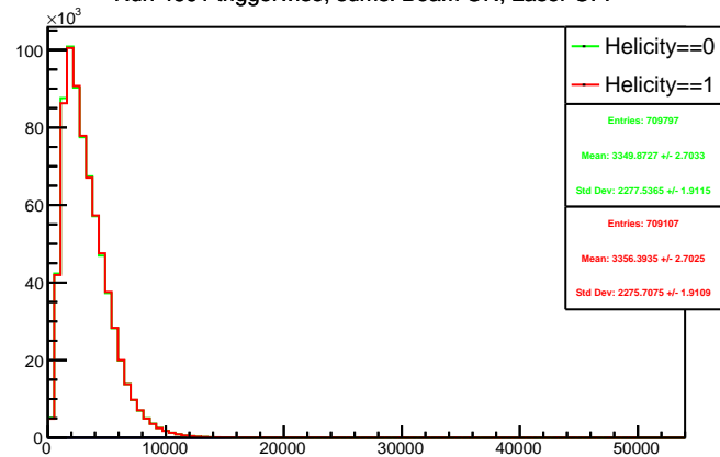
Run 4601 triggerwise, sums: Beam ON, Laser OFF
