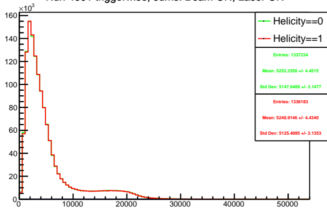
Run 4601 triggerwise, sums: Beam ON, Laser ON
