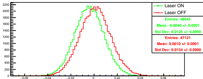
Run 4603 quartetwise, asym0: Beam ON
