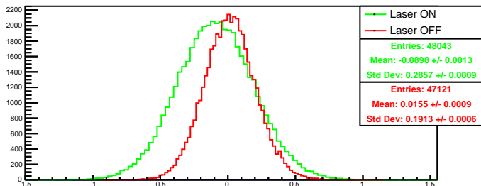
Run 4603 quartetwise, diff0: Beam ON
