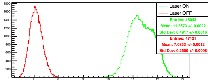
Run 4603 quartetwise, negH0: Beam ON
