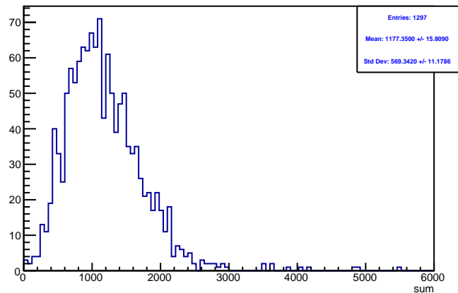
Run 4603 triggerwise, sums: Beam OFF
