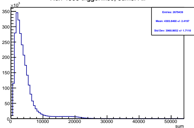
Run 4603 triggerwise, sums: All
