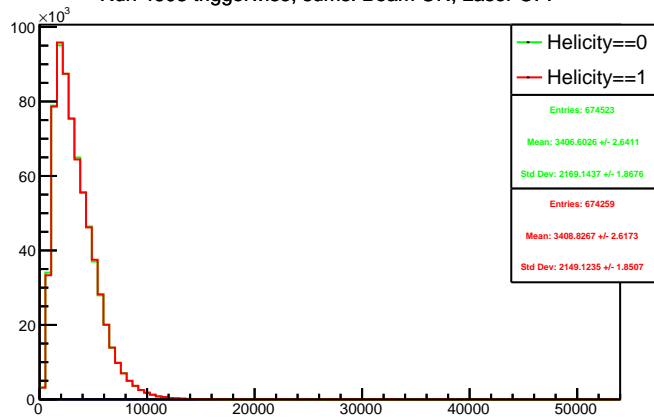
Run 4603 triggerwise, sums: Beam ON, Laser OFF
