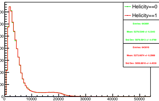
Run 4603 triggerwise, sums: Beam ON, Laser ON
