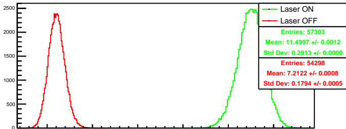
Run 4607 quartetwise, posH0: Beam ON
