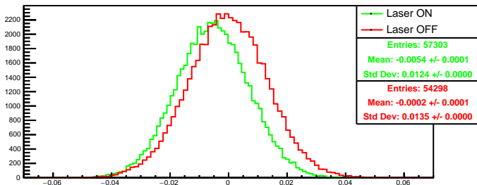
Run 4607 quartetwise, asym0: Beam ON
