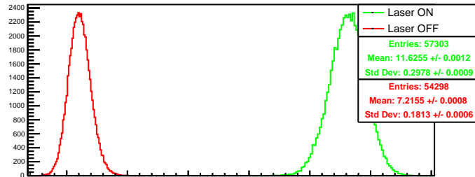
Run 4607 quartetwise, negH0: Beam ON
