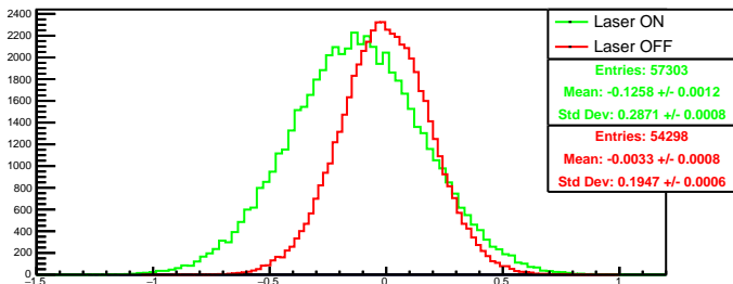
Run 4607 quartetwise, diff0: Beam ON
