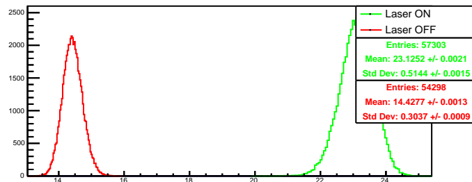
Run 4607 quartetwise, summ0: Beam ON
