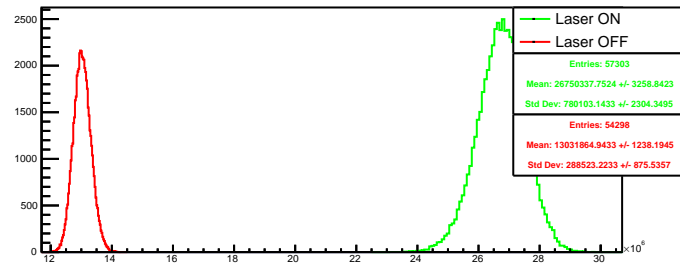
Run 4607 quartetwise, negH4: Beam ON
