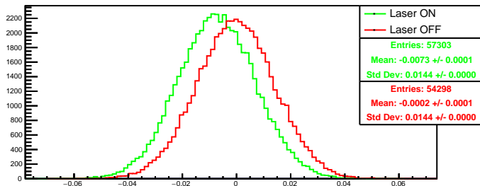
Run 4607 quartetwise, asym4: Beam ON
