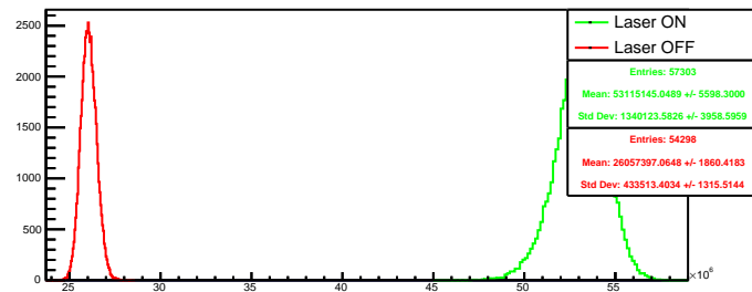
Run 4607 quartetwise, summ4: Beam ON
