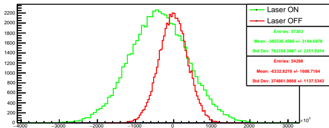
Run 4607 quartetwise, diff4: Beam ON
