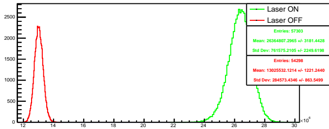
Run 4607 quartetwise, posH4: Beam ON
