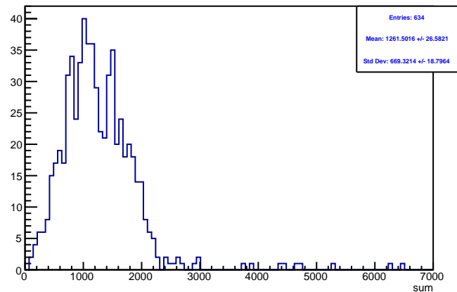
Run 4607 triggerwise, sums: Beam ON, Laser OFF
