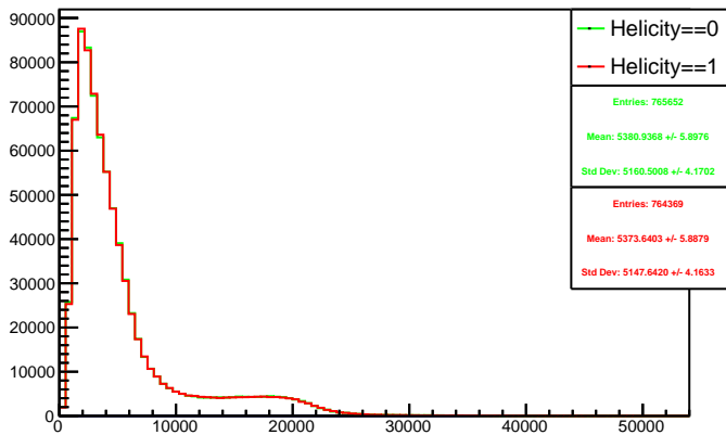
Run 4607 triggerwise, sums: Beam ON, Laser ON
