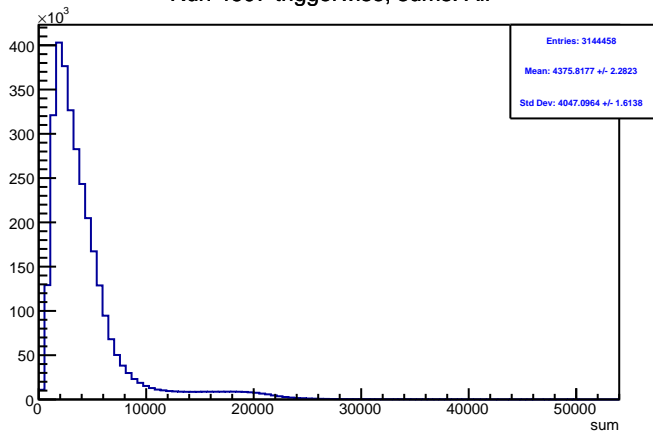
Run 4607 triggerwise, sums: All
