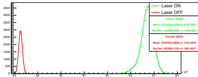
Run 4608 quartetwise, summ4: Beam ON
