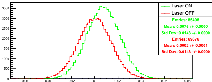
Run 4608 quartetwise, asym4: Beam ON
