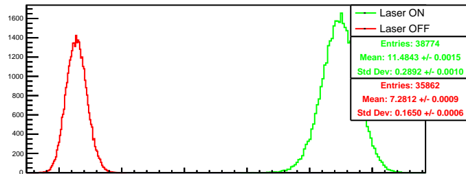
Run 4609 quartetwise, negH0: Beam ON
