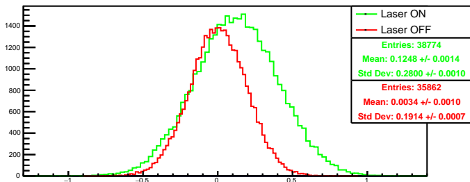
Run 4609 quartetwise, diff0: Beam ON
