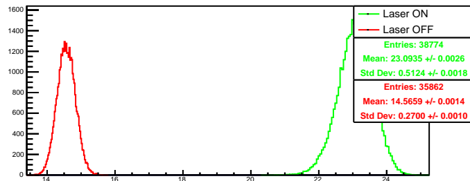
Run 4609 quartetwise, summ0: Beam ON
