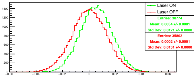
Run 4609 quartetwise, asym0: Beam ON
