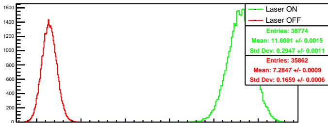
Run 4609 quartetwise, posH0: Beam ON
