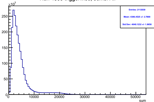
Run 4609 triggerwise, sums: All
