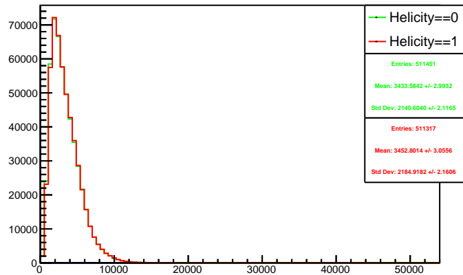
Run 4609 triggerwise, sums: Beam ON, Laser OFF
