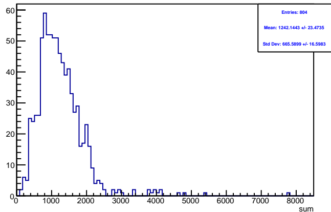
Run 4609 triggerwise, sums: Beam ON, Laser OFF
