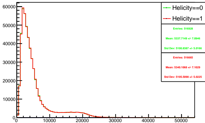
Run 4609 triggerwise, sums: Beam ON, Laser ON
