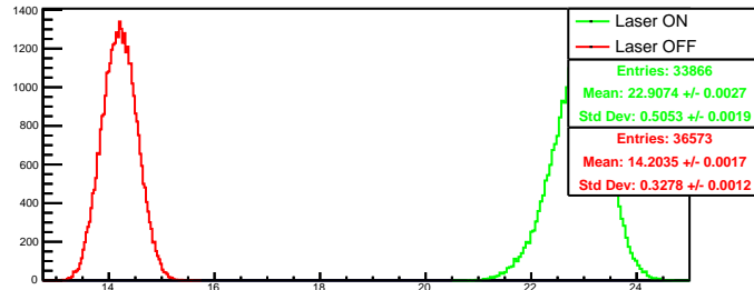
Run 4610 quartetwise, summ0: Beam ON
