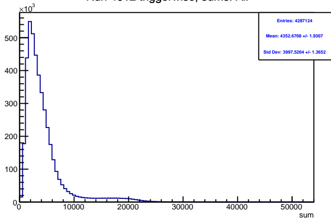
Run 4612 triggerwise, sums: All
