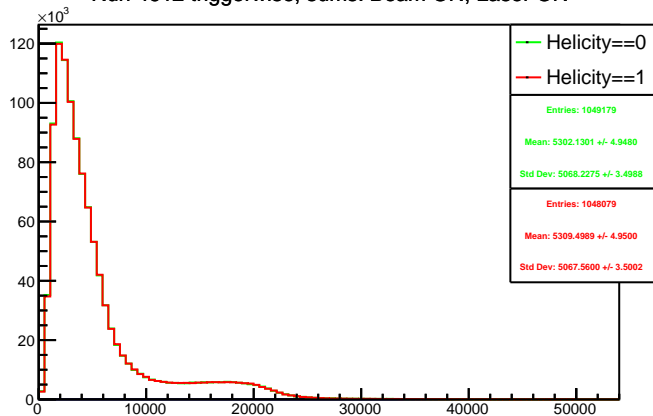
Run 4612 triggerwise, sums: Beam ON, Laser ON
