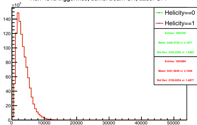
Run 4612 triggerwise, sums: Beam ON, Laser OFF
