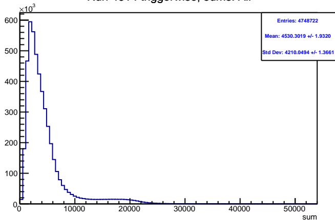
Run 4614 triggerwise, sums: All
