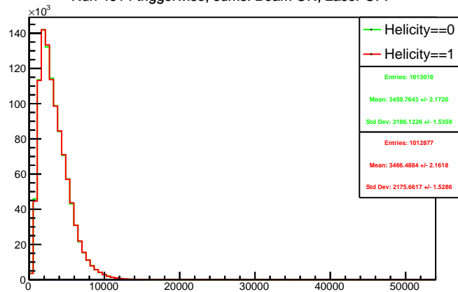
Run 4614 triggerwise, sums: Beam ON, Laser OFF
