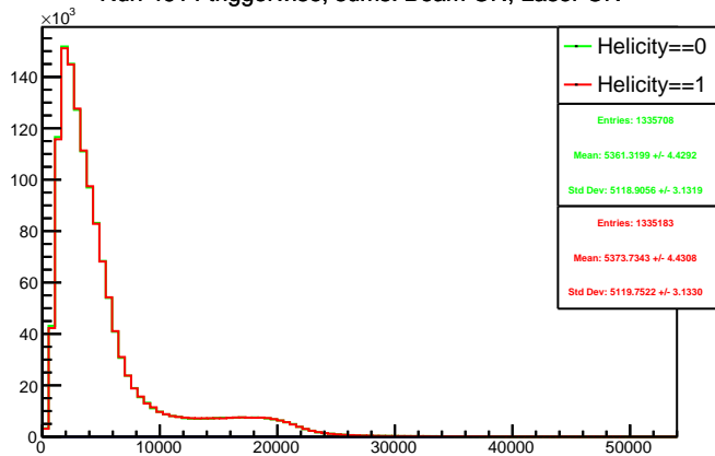
Run 4614 triggerwise, sums: Beam ON, Laser ON
