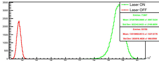
Run 4615 quartetwise, negH4: Beam ON
