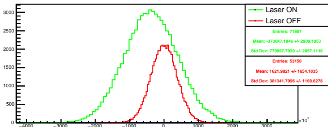
Run 4615 quartetwise, diff4: Beam ON
