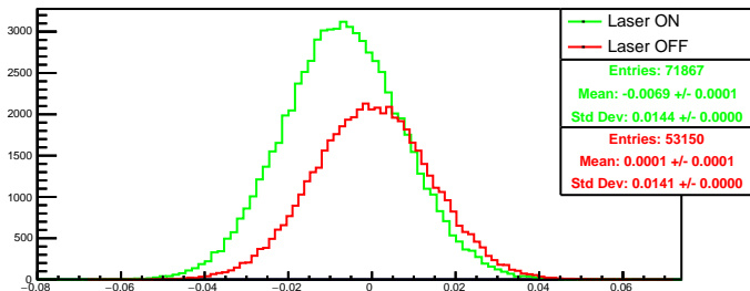
Run 4615 quartetwise, asym4: Beam ON
