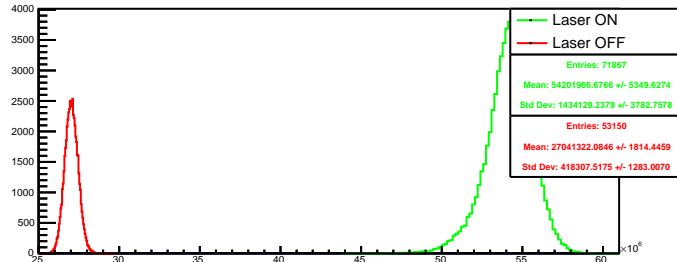
Run 4615 quartetwise, summ4: Beam ON
