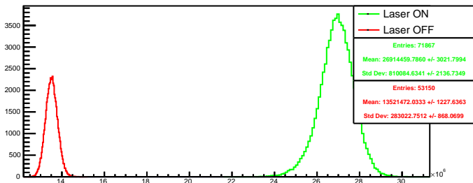
Run 4615 quartetwise, posH4: Beam ON
