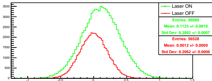
Run 4621 quartetwise, diff0: Beam ON
