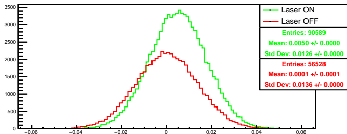
Run 4621 quartetwise, asym0: Beam ON
