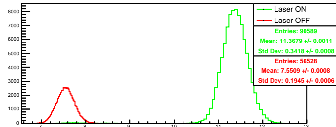
Run 4621 quartetwise, negH0: Beam ON
