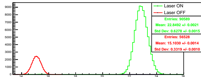
Run 4621 quartetwise, summ0: Beam ON
