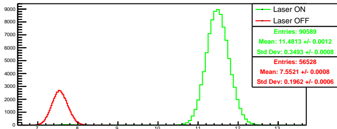
Run 4621 quartetwise, posH0: Beam ON
