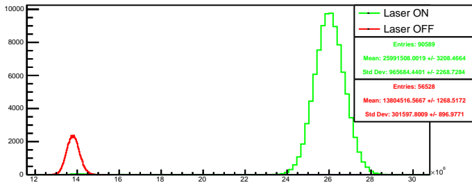
Run 4621 quartetwise, posH4: Beam ON
