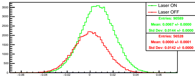
Run 4621 quartetwise, asym4: Beam ON
