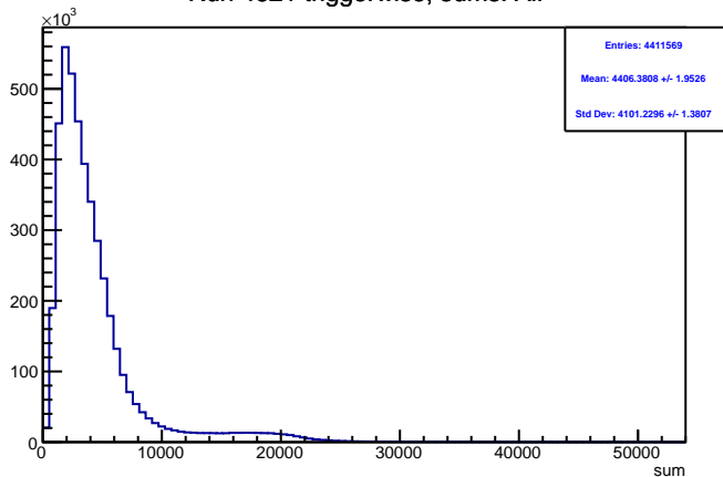
Run 4621 triggerwise, sums: All
