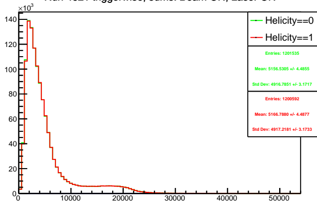
Run 4621 triggerwise, sums: Beam ON, Laser ON
