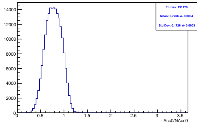
Run 4622 mpwise, acc0: Beam ON, Laser OFF
