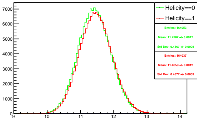
Run 4622 mpwise, acc0: Beam ON, Laser ON
