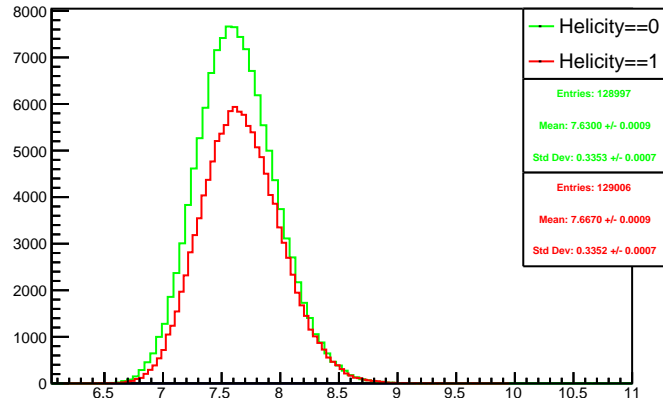
Run 4622 mpwise, acc0: Beam ON, Laser OFF
