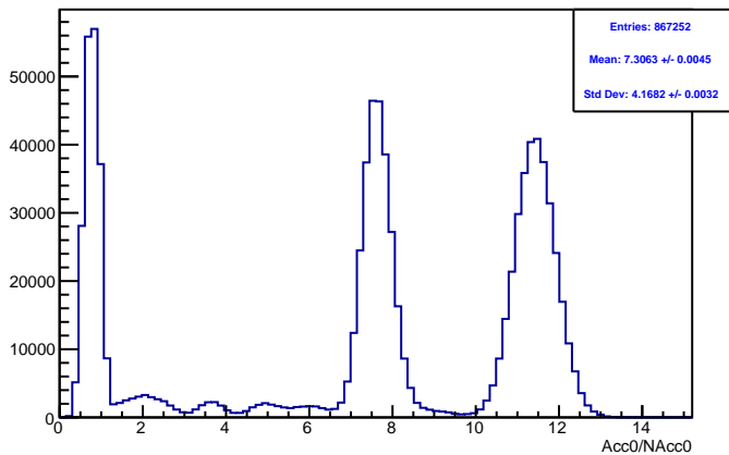
Run 4622 mpwise, acc0: Beam ON, Laser ON
