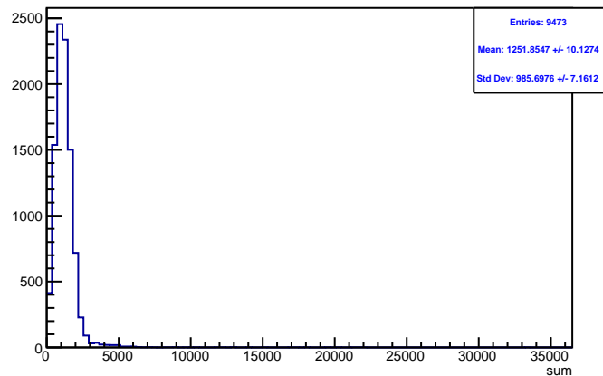
Run 4622 triggerwise, sums: Beam ON, Laser OFF
