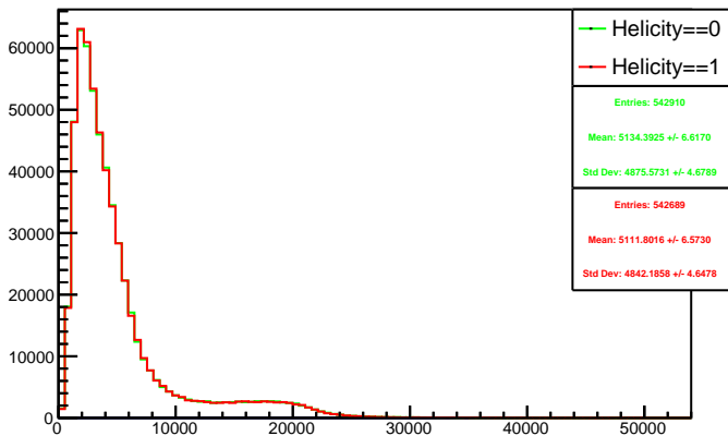
Run 4622 triggerwise, sums: Beam ON, Laser ON
