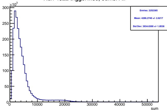
Run 4622 triggerwise, sums: All
