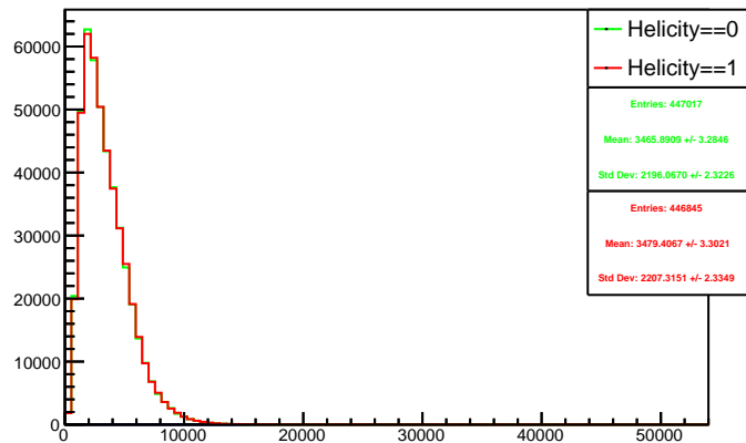
Run 4622 triggerwise, sums: Beam ON, Laser OFF
