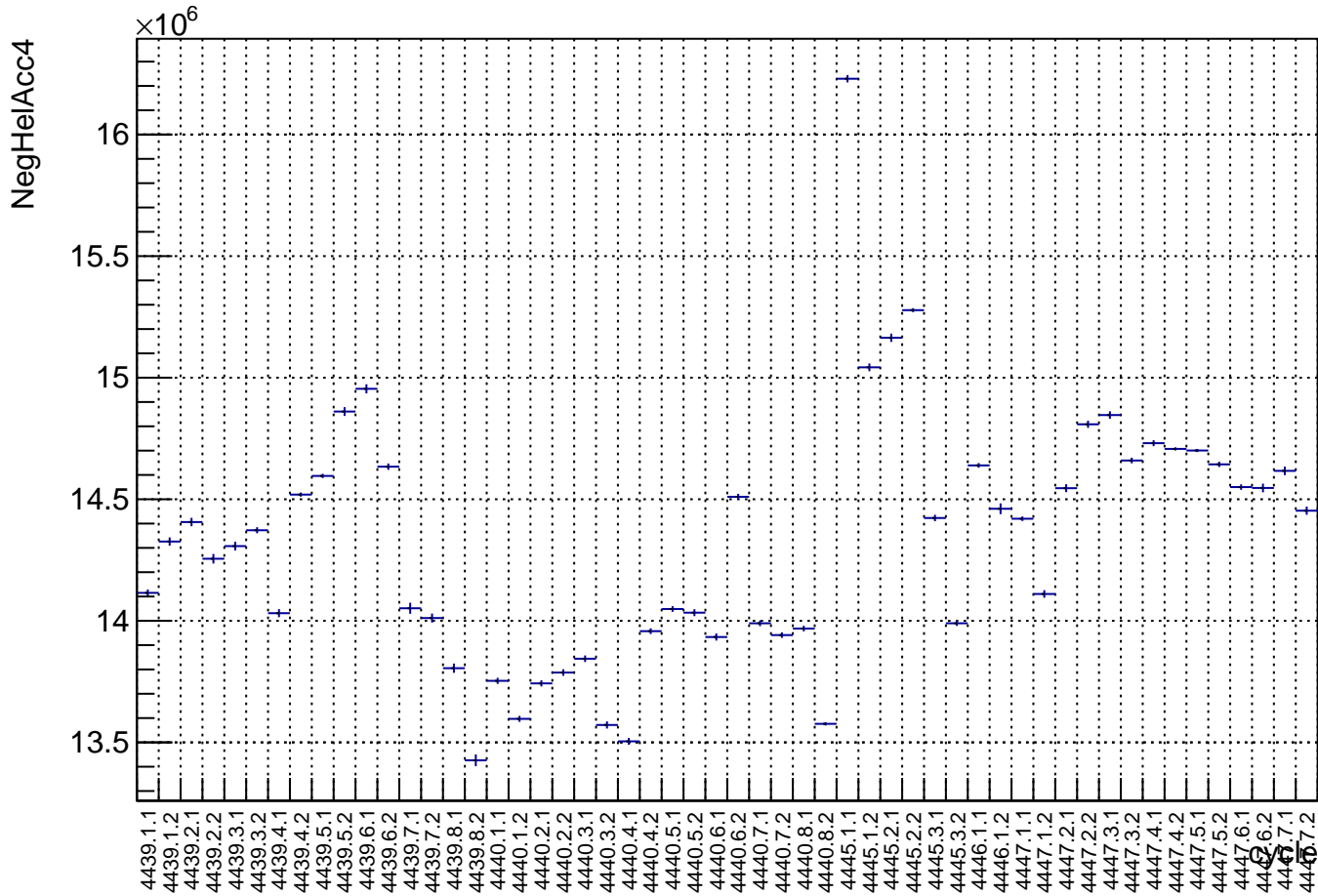
Laser NegHel Background by cycle: snail14 (Acc4)
