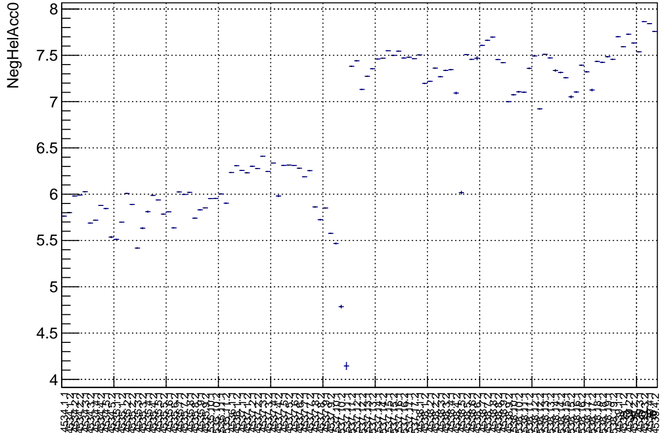
Laser NegHel Background by cycle: snail26 (Acc0)
