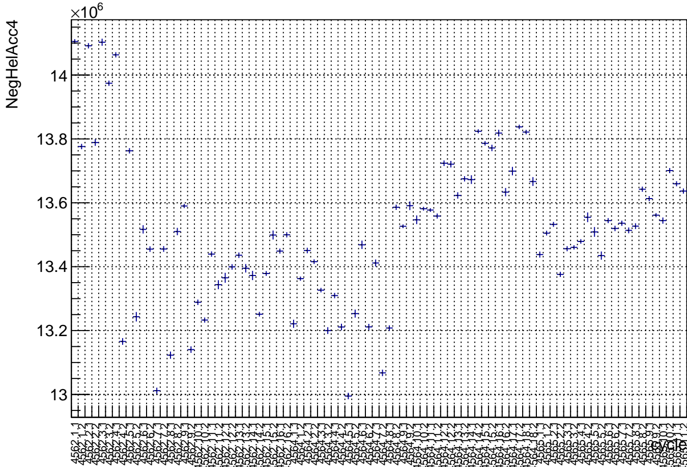
Laser NegHel Background by cycle: snail31 (Acc4)
