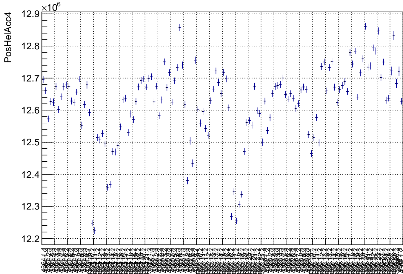
Laser PosHel Background by cycle: snail5 (Acc4)
