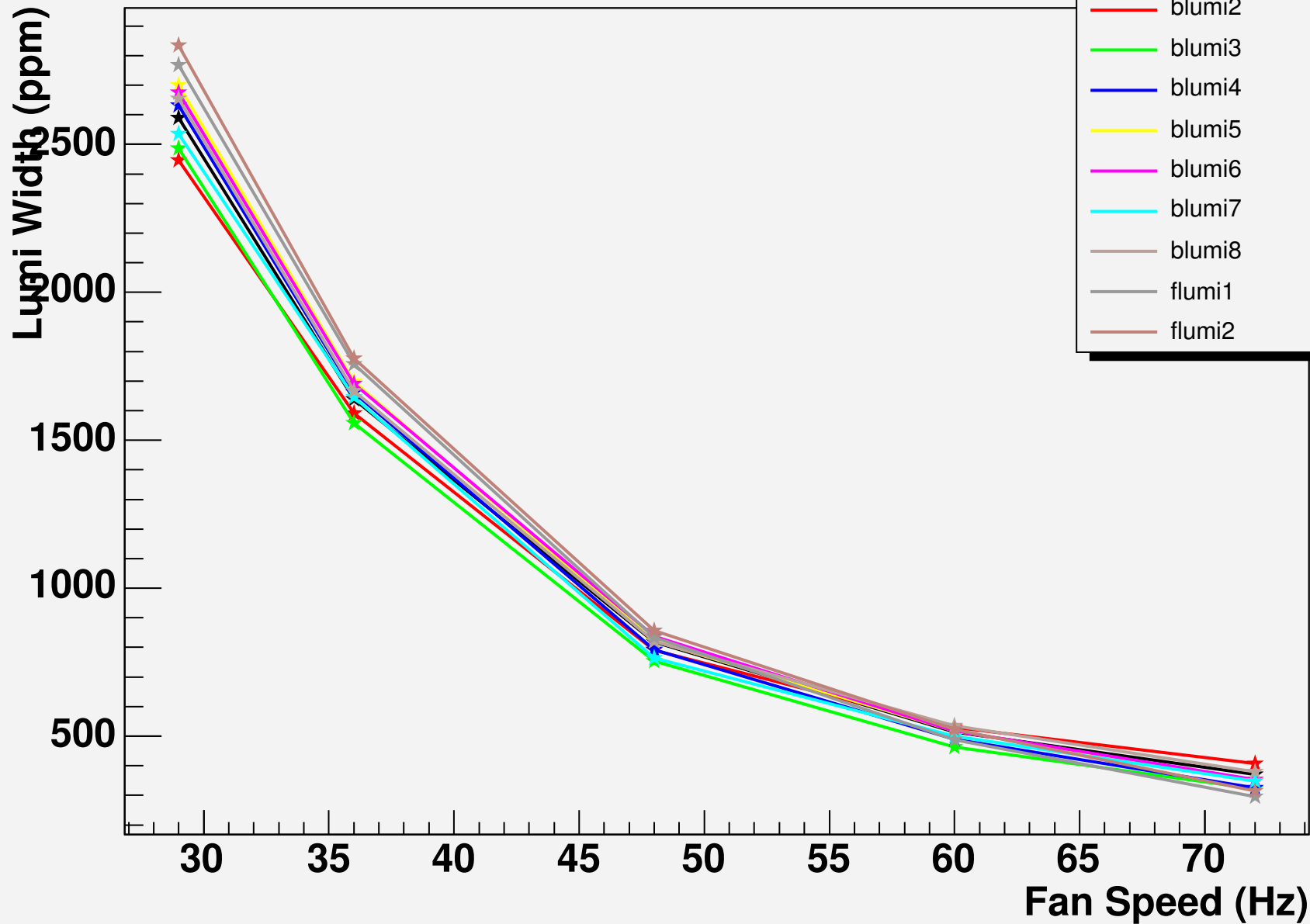
Lumi Widths vs. Fan Speed with 0.8*0.8 mm raster at 36uA
