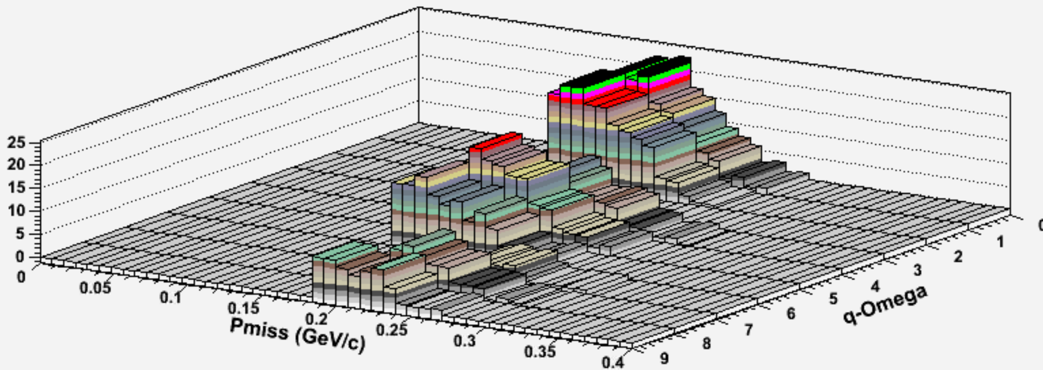
REDUCED CROSS SECTION (DATA) KIN D-
