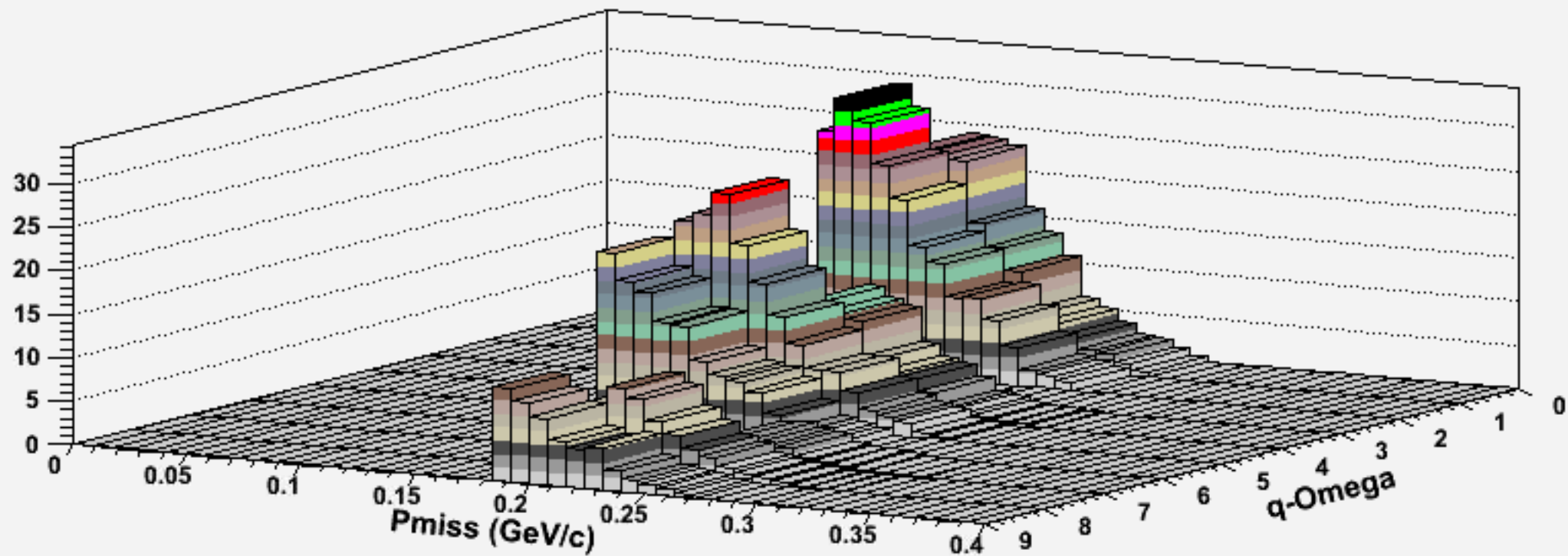
REDUCED CROSS SECTION (MCEEP) KIN D-
