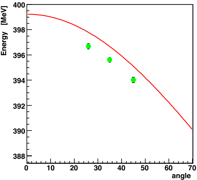
12C elastic scattering
