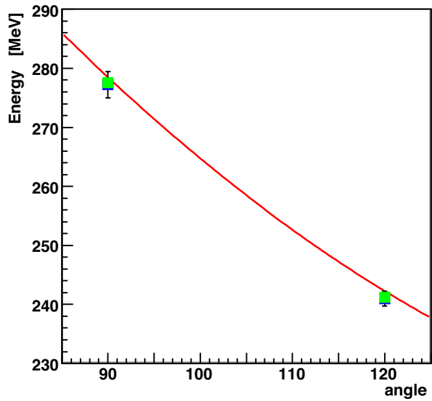
1H elastic scattering
