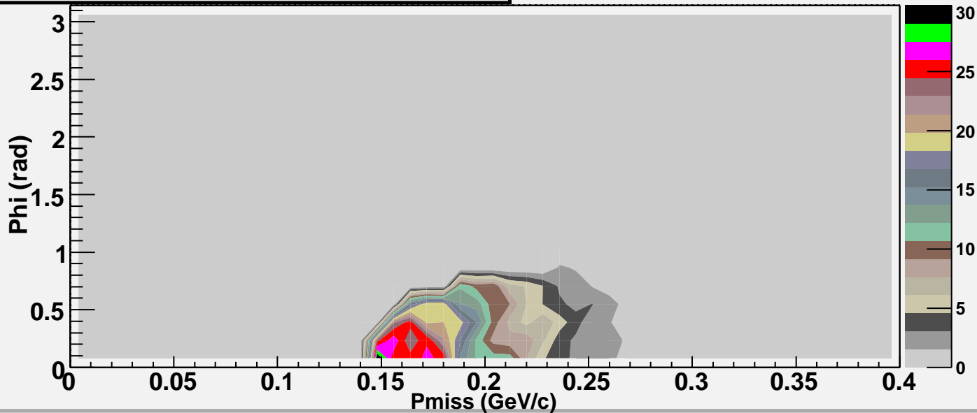
REDUCED CROSS SECTION (MCEEP) – KIN D–
