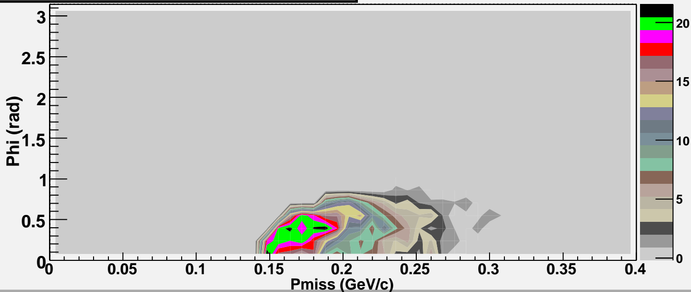
REDUCED CROSS SECTION (DATA) – KIN D–
