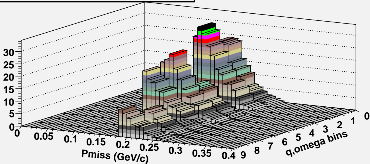
REDUCED CROSS SECTION (MCEEP) KIN D-
