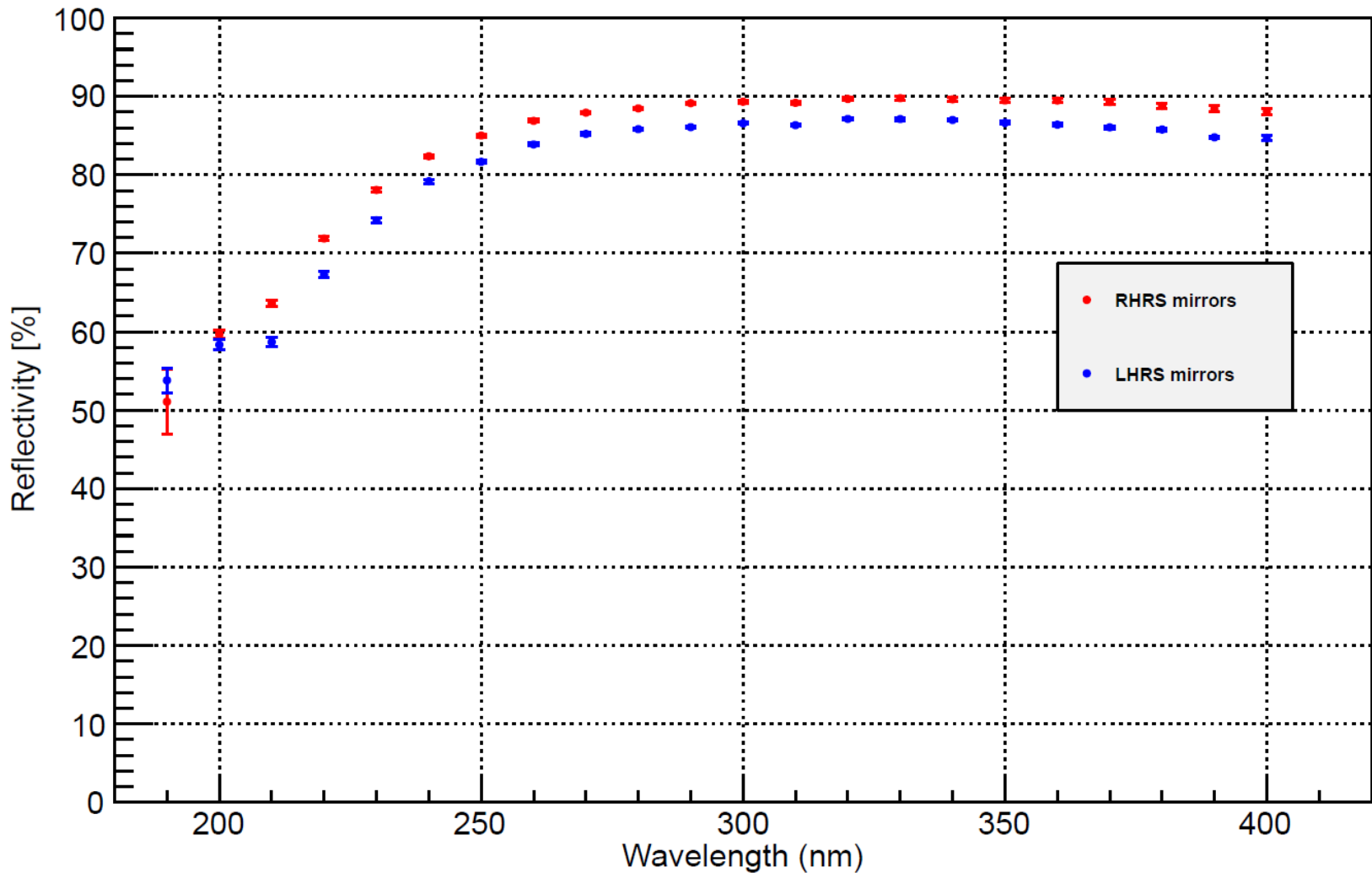
Comparison of Average Reflectivity of RHRS and LHRS Mirrors
