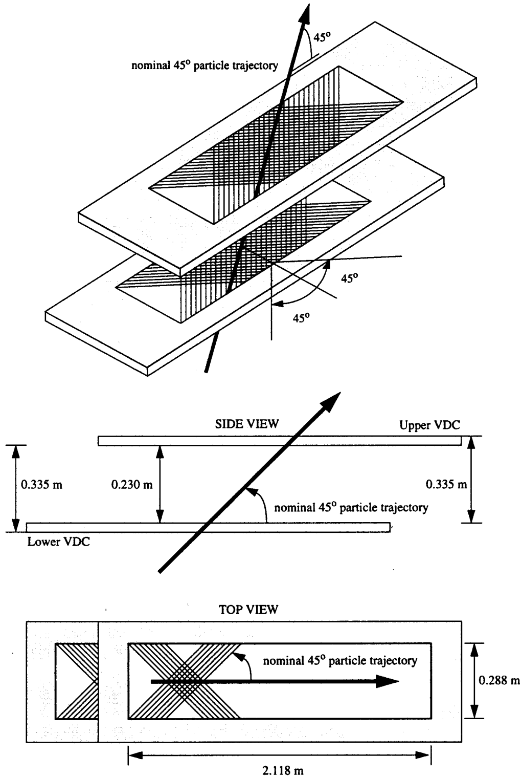
Fig. 1. Schematic layout of the VDCs (not to scale). The rectangular area of each wire frame aperture is 2.118\text{ m} \times 0.288\text{ m} (see 3.2.1). The U and V sense wires are orthogonal to each other and lie in the horizontal plane of the laboratory. They are inclined at an angle of 45^\circ with respect to both the dispersive and non-dispersive directions. The lower VDC coincides (essentially) with the spectrometer focal plane. The vertical offset between like wire planes is 0.335\text{ m} .
