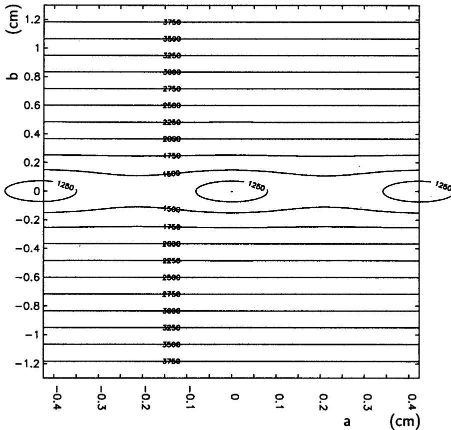
Fig. 4. GARFIELD model [13,14] of the negative high voltage contours within a drift cell. The contours are labelled in V. See Fig. 3 for the definition of the coordinates 'a' and 'b'. In the region close to the sense wire, the equipotential surfaces undergo a transition from parallel to elliptical.
