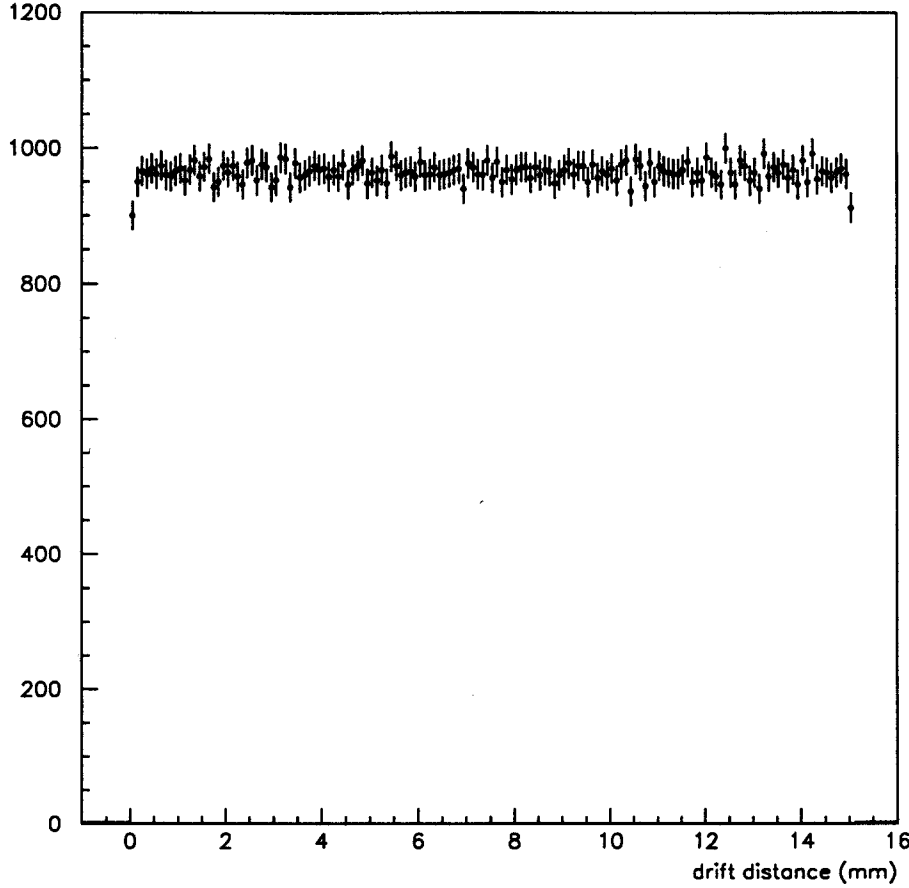
Fig. 20. The drift-distance spectrum corresponding to the drift-time spectrum shown in Fig. 17. The mapping algorithm is the lookup table illustrated in Fig. 19. The bins are 100\ \mu\text{m} .
