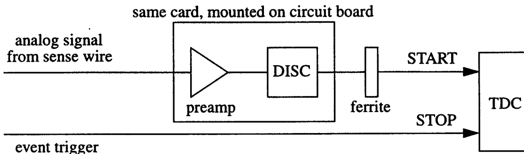
Fig. 11. A block diagram of the sense wire electronics. The preamp/discriminator cards are mounted on the circuit boards. Signals proceed to the TDCs via 10-m long, twisted-pair cables. Each wire has its own TDC channel. The TDCs have 0.5 ns/channel resolution and are operated in common stop mode.
