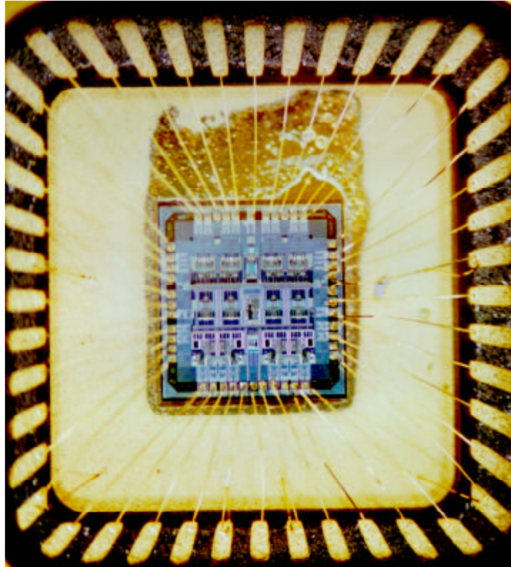
Figure 7: Microphoto of the definitive die bonded to a ceramic case.
