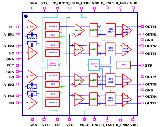
Figure 1: Block diagram of the ASIC.
