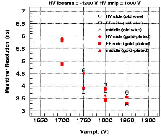
Figure 4: Meantimer resolution for different beam positions along the wires and different amplification.
