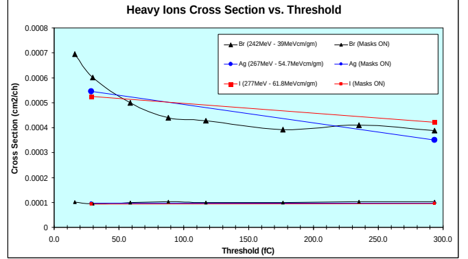
Figure 6: Heavy ions cross-section versus threshold.
