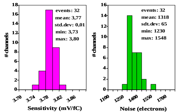
Figure 2: Sensitivity and noise of bare ASIC.
