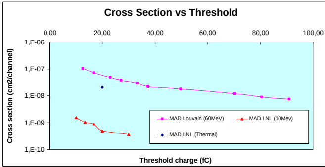
Figure 5: Fast and slow neutrons cross-section versus threshold.
