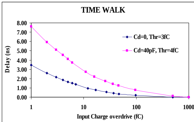
Figure 3: Time walk of the bare chip with 2 input configurations.
