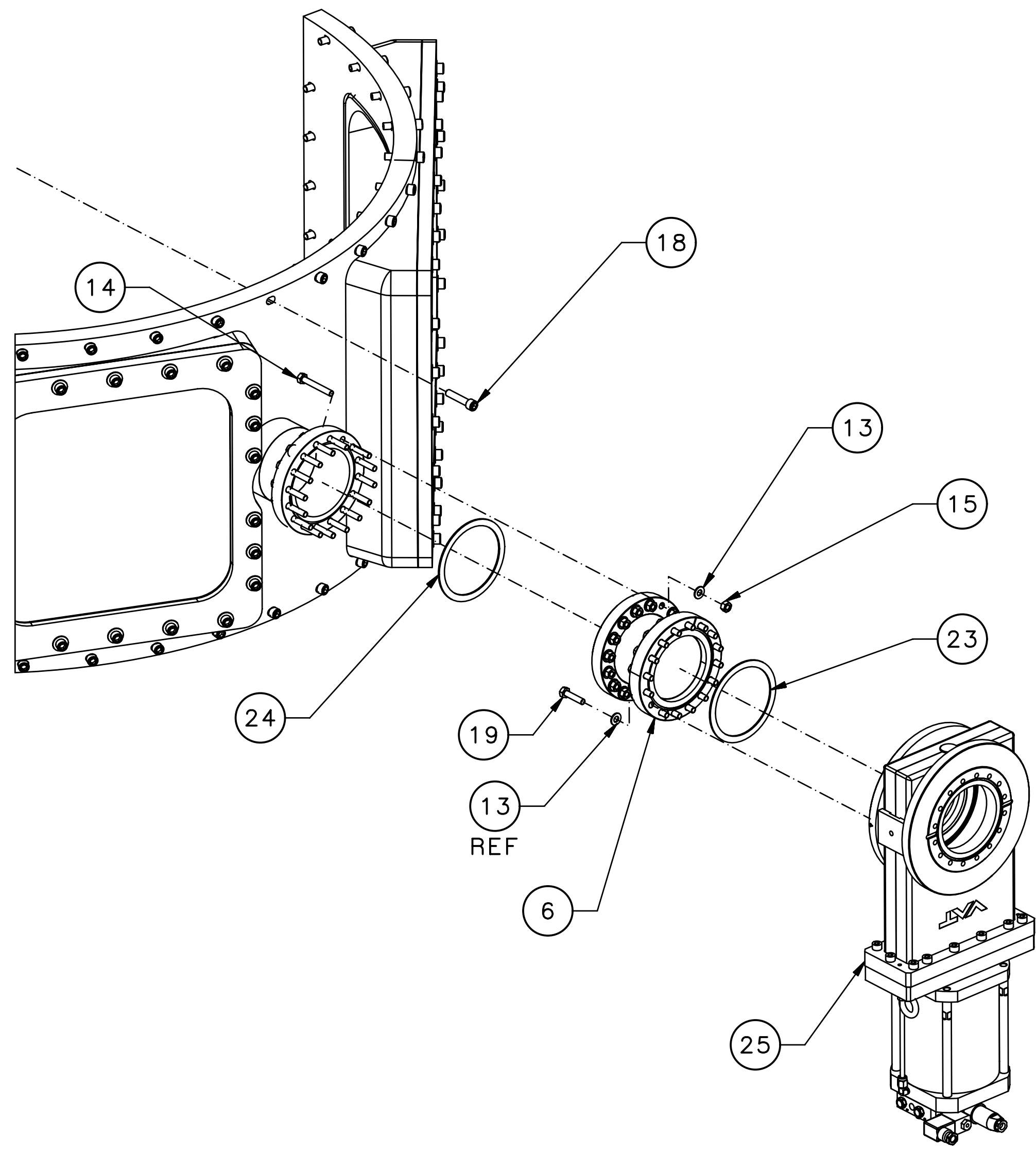
DETAIL VIEW 1-3E SCALE 3:16
