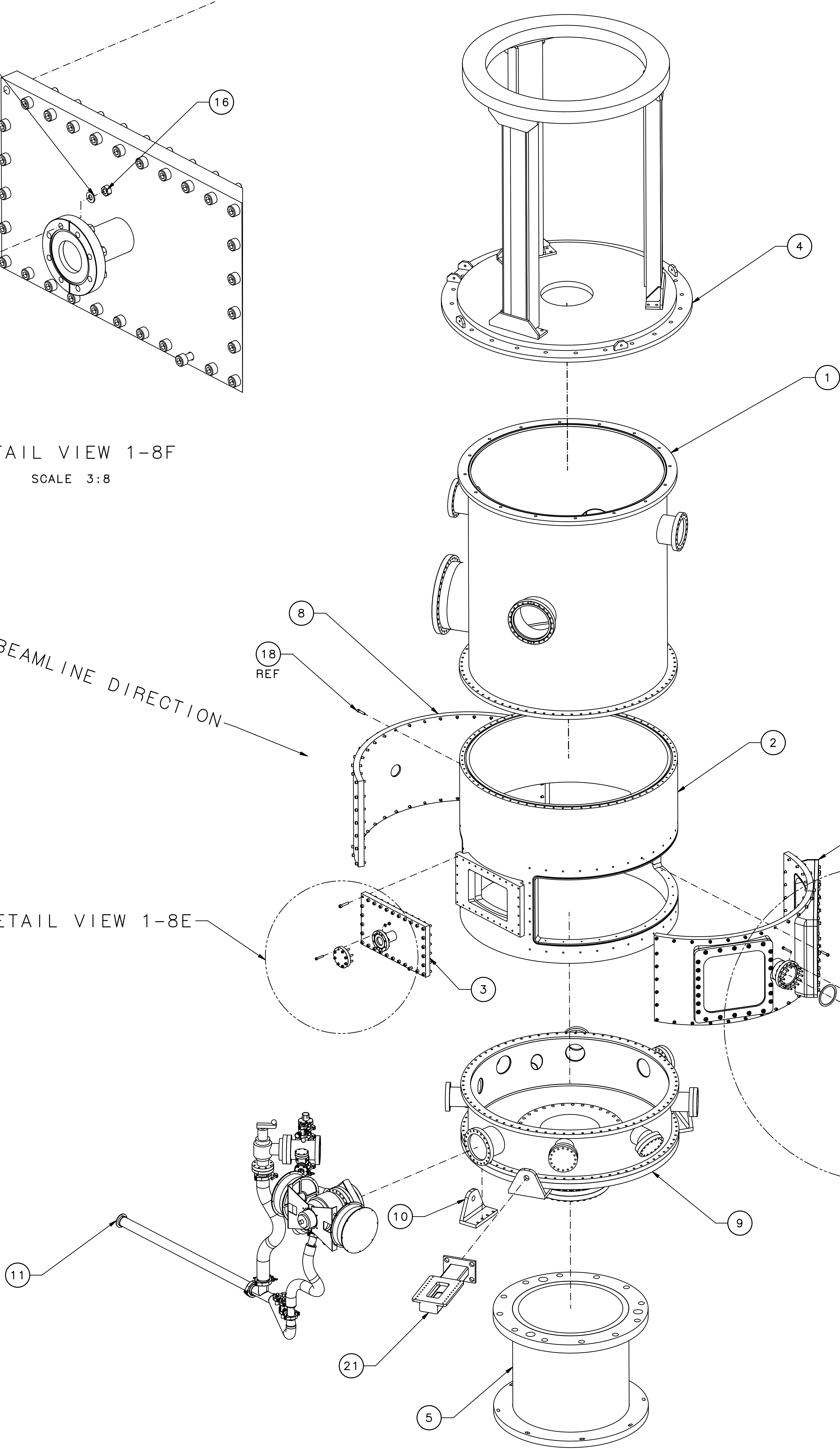
EXPLODED VIEW 1-6A
