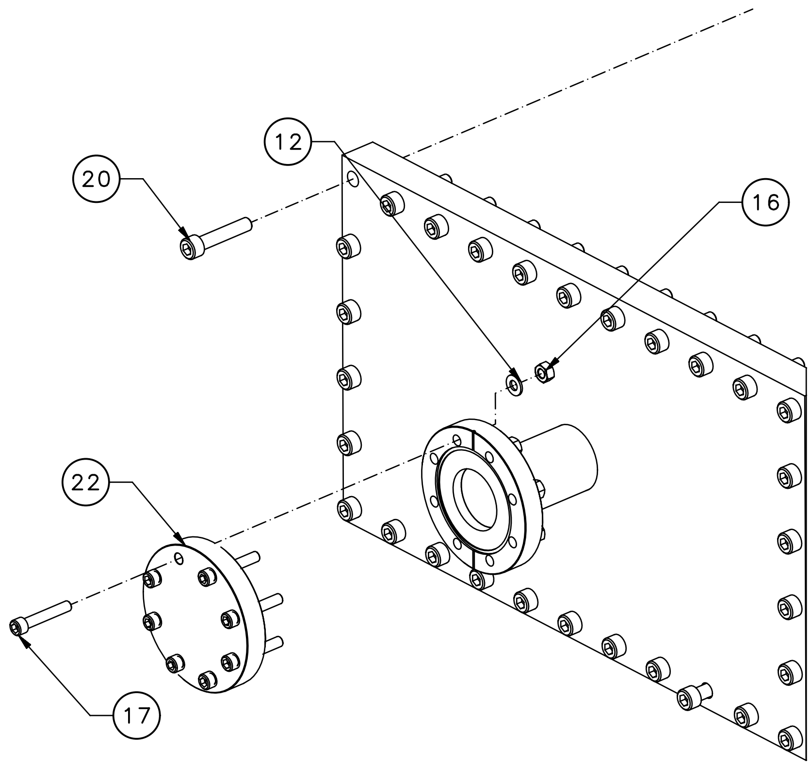
DETAIL VIEW 1-8F SCALE 3:8
