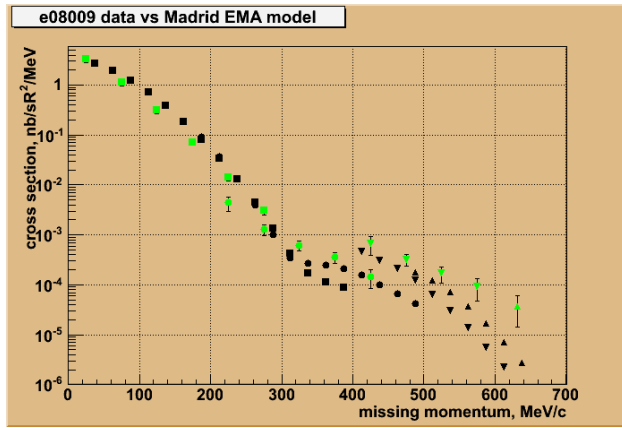
Figure 25: E08009 Data in green compared to EMA Madrid theoretical calculations in black. Squares are for the 153 MeV/c setting, circles are for 353 MeV/c setting, inverted triangles are for the 466 MeV/c setting and triangles are for the 632 MeV/c setting.
