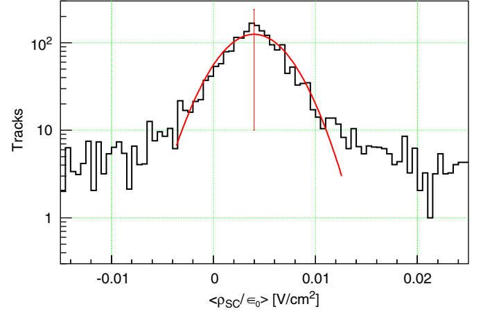
Fig. 2. Observed space charge density (averaged over the volume of the TPC) determined from individual tracks in a single high-multiplicity event. The mean of a Gaussian peak (formed from primaries) is fit to extract \rho_{SC}^{obs} for that event.
