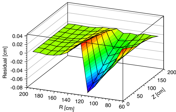
Fig. 4. Residuals of TPC tracks over R and Z in a selection of events acquired during high luminosity before (left) and after (right) leakage distortion corrections. The gap between inner and outer wire chambers is at R \approx 122 cm.
