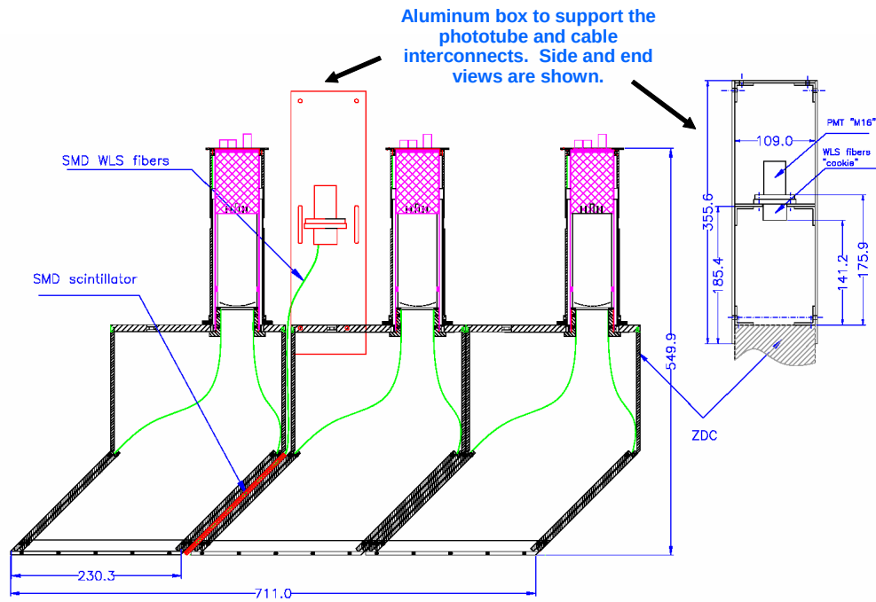
FIG. 6: The SMD fits between the existing ZDC modules.
