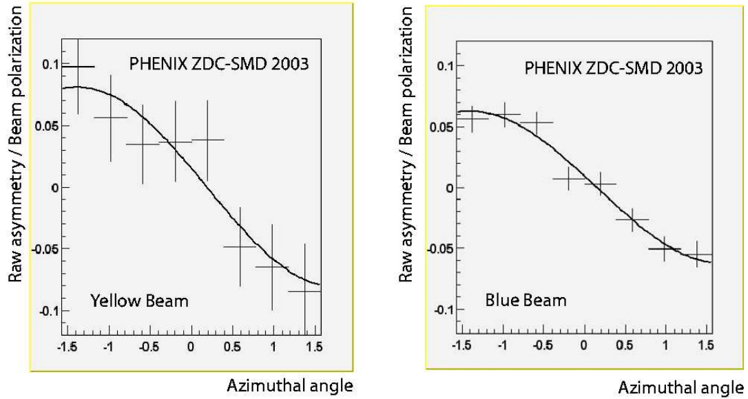
FIG. 3: PHENIX transverse raw asymmetries divided by the respective beam polarization for forward neutron production for Yellow (left) and Blue (right) spin sorting using the PHENIX ZDC-SMD detector system as a function of the reconstructed azimuthal angle in the range of -\pi/2 to \pi/2 , ignoring sign conventions in A_N .
