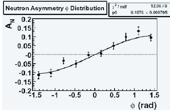
FIG. 2: Preliminary result of the measured neutron asymmetry as a function of the reconstructed azimuthal angle \phi by the Local Polarimetry (PHENIX) collaboration using a Lead-Tungstate ( \text{PbWO}_4 ) crystal electromagnetic calorimeter.
