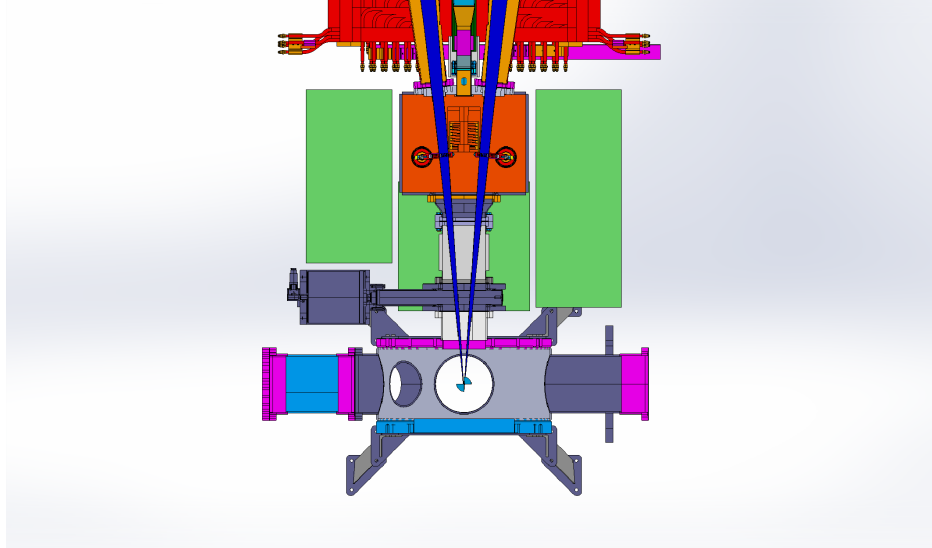
Figure 4: Top View of horizontal midplane cut through the pivot region.
