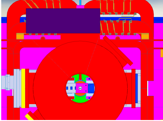
Figure 11: Beam's eye view from front of the scattering chamber, showing location of the target sky-shine shield relative to the scattering chamber.
