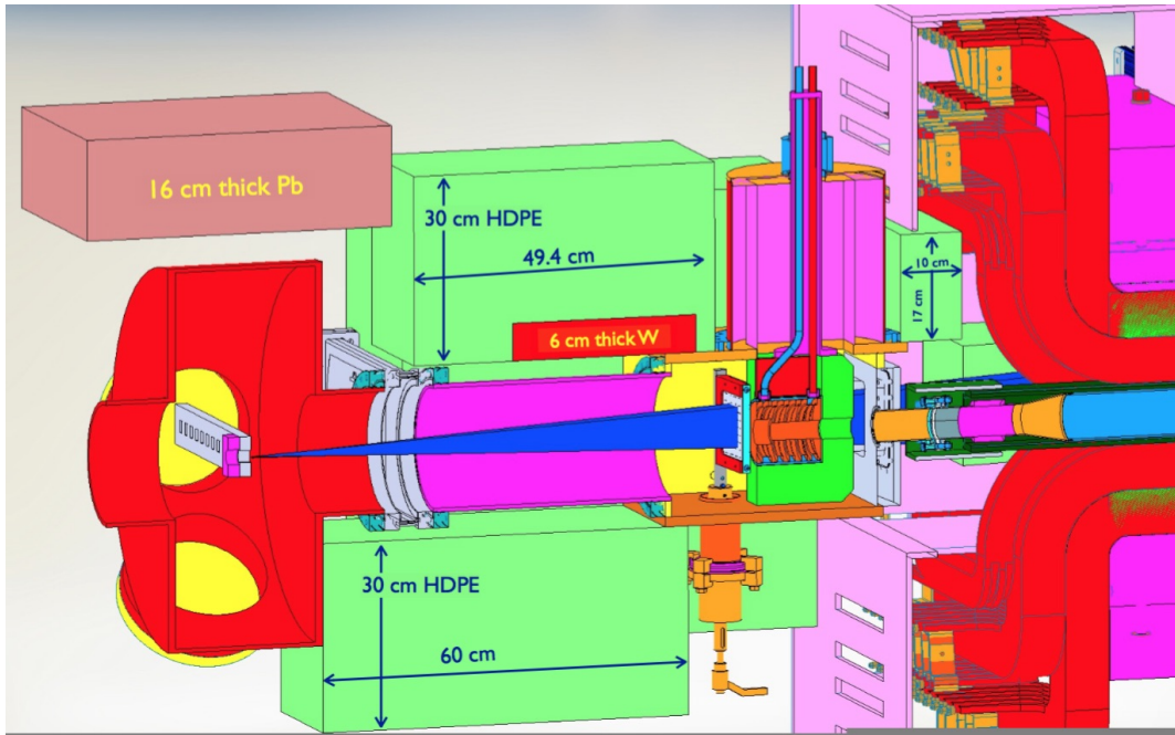
Figure 12: Perspective view (with vertical midplane section) of the pivot region with HDPE shielding.
