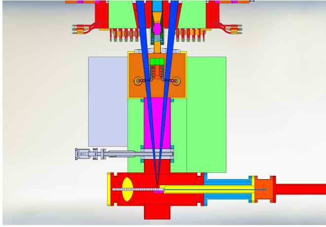
Figure 4: Top View of horizontal midplane cut through the pivot region.
