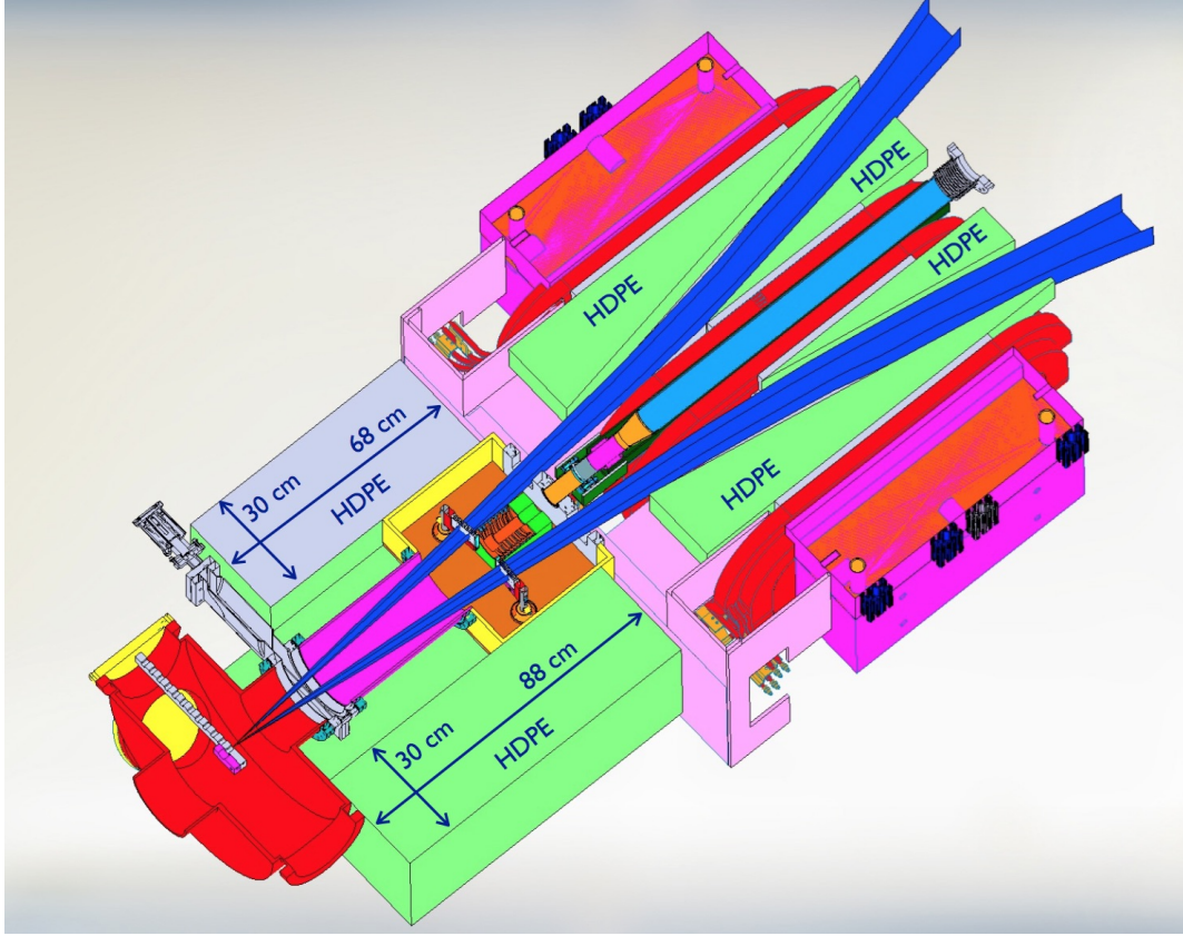
Figure 13: Perspective view (with horizontal midplane section) of the pivot region with HDPE shielding.
