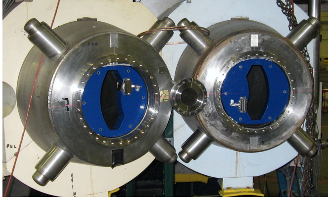
Figure 10: Q1 acceptance collimators installed for PREX-I.
