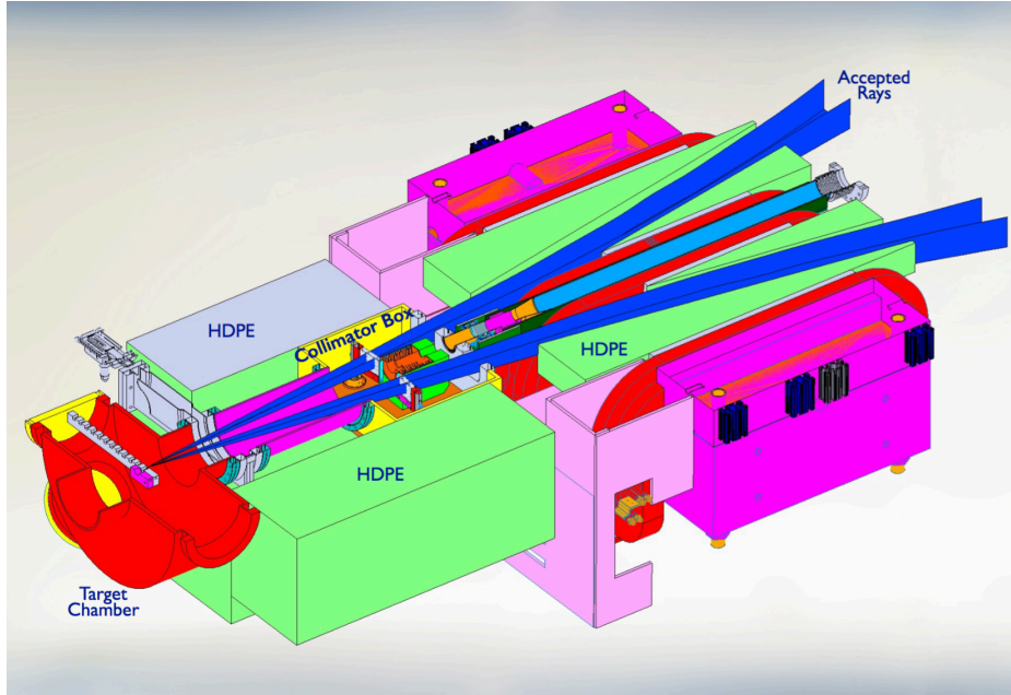
Figure 2: Perspective view of the pivot region with midplane cut, from UVa SOLIDWORKS CAD model.
