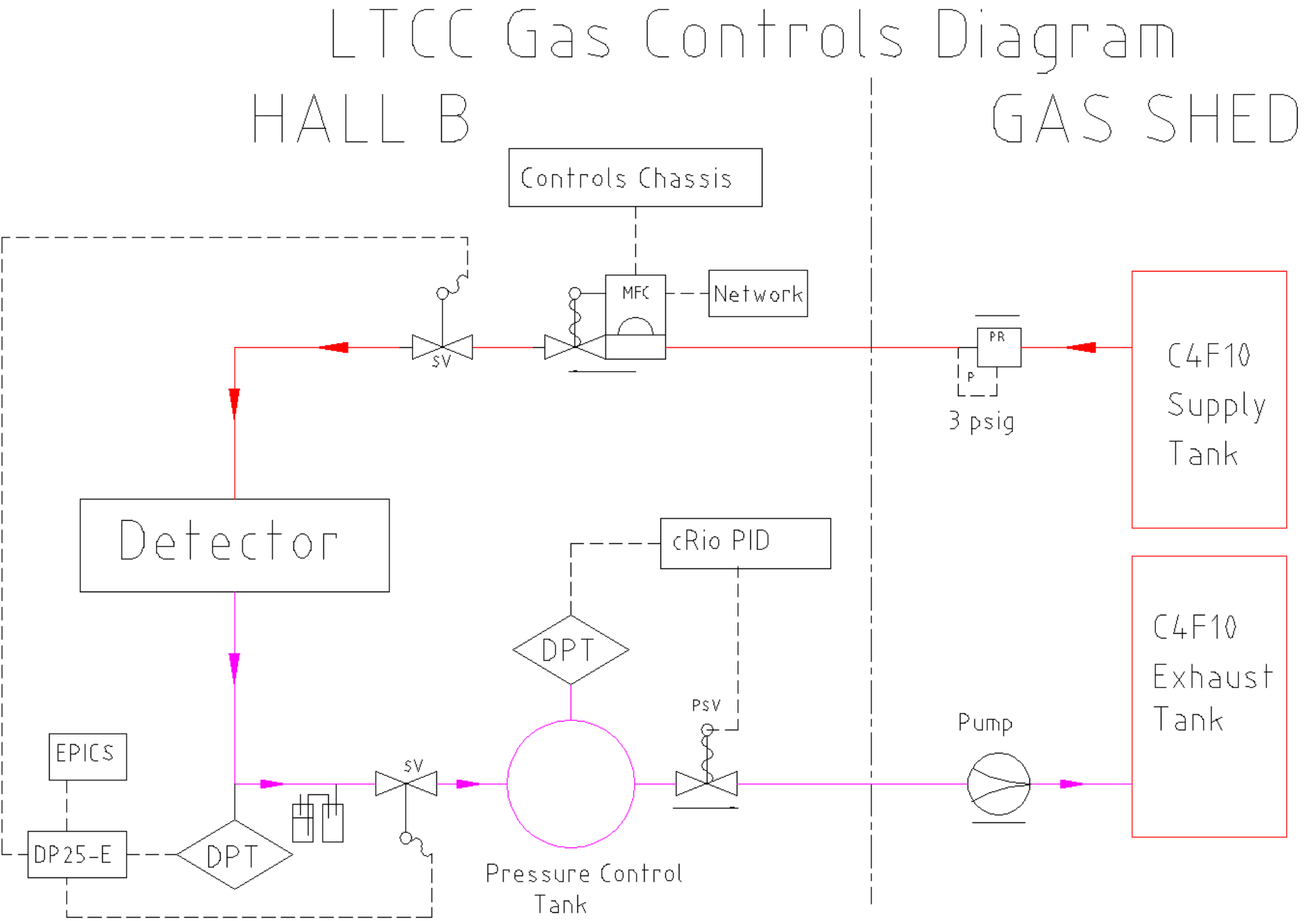
CLAS Cerenkov Gas System Controls Diagram Physics DSG Group George Jacobs 03-28-2016
