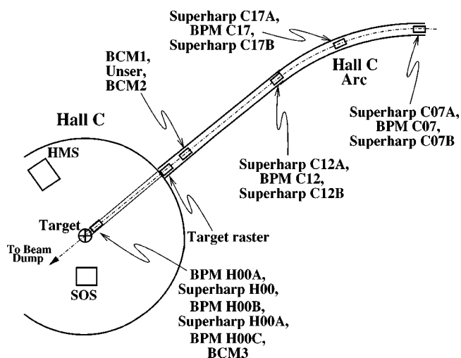
FIG. 3. Schematic of the Hall C beamline.
