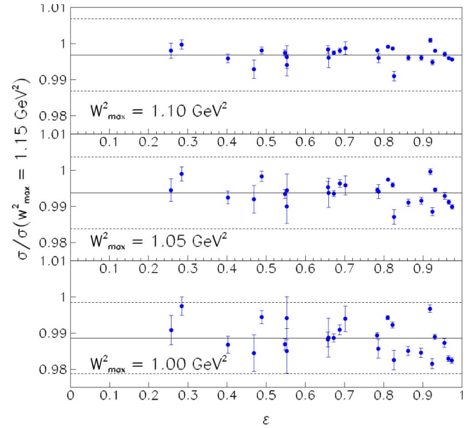
FIG. 13. (Color online) Ratio of the cross section calculated with a cutoff in the tail integration of W^2 = 1.10 \text{ GeV}^2 (top), W^2 = 1.05 \text{ GeV}^2 (middle), and W^2 = 1.00 \text{ GeV}^2 (bottom), relative to a cutoff of W^2 = 1.15 \text{ GeV}^2
