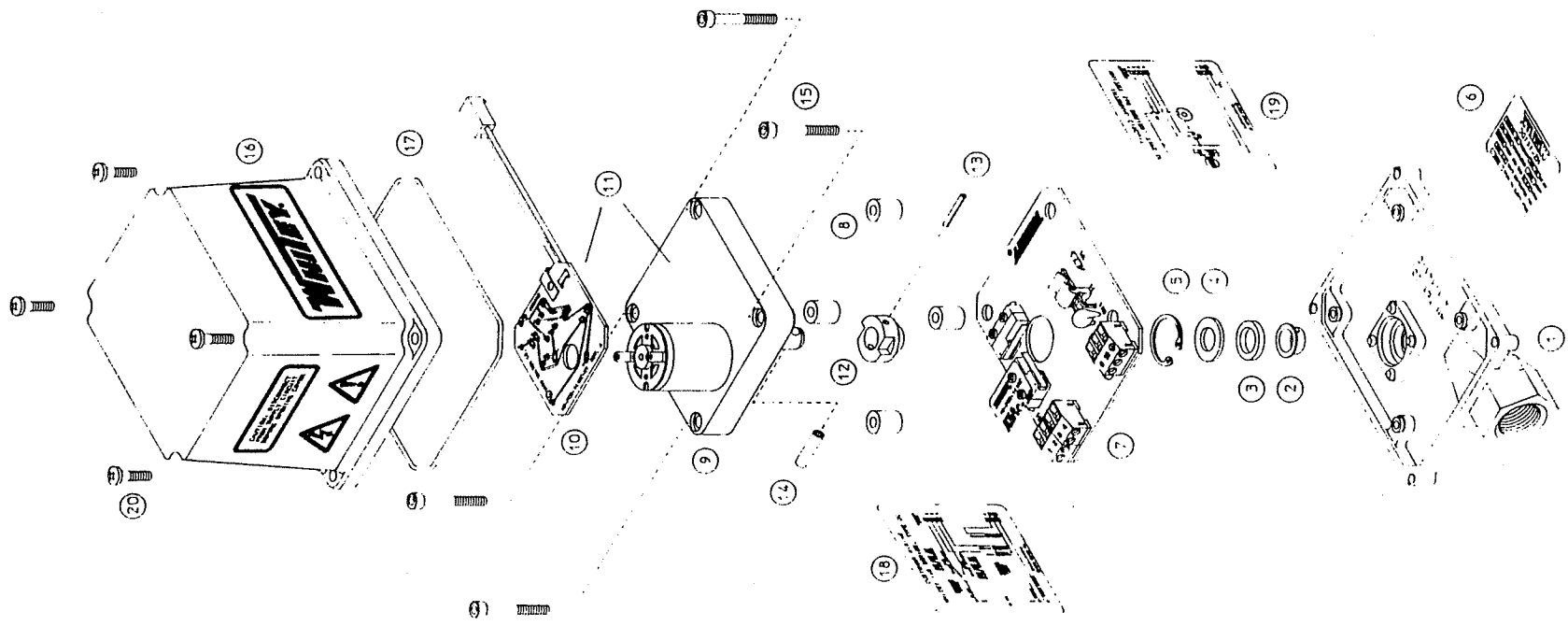
Exploded View of the 141 Series Type DC Actuator
