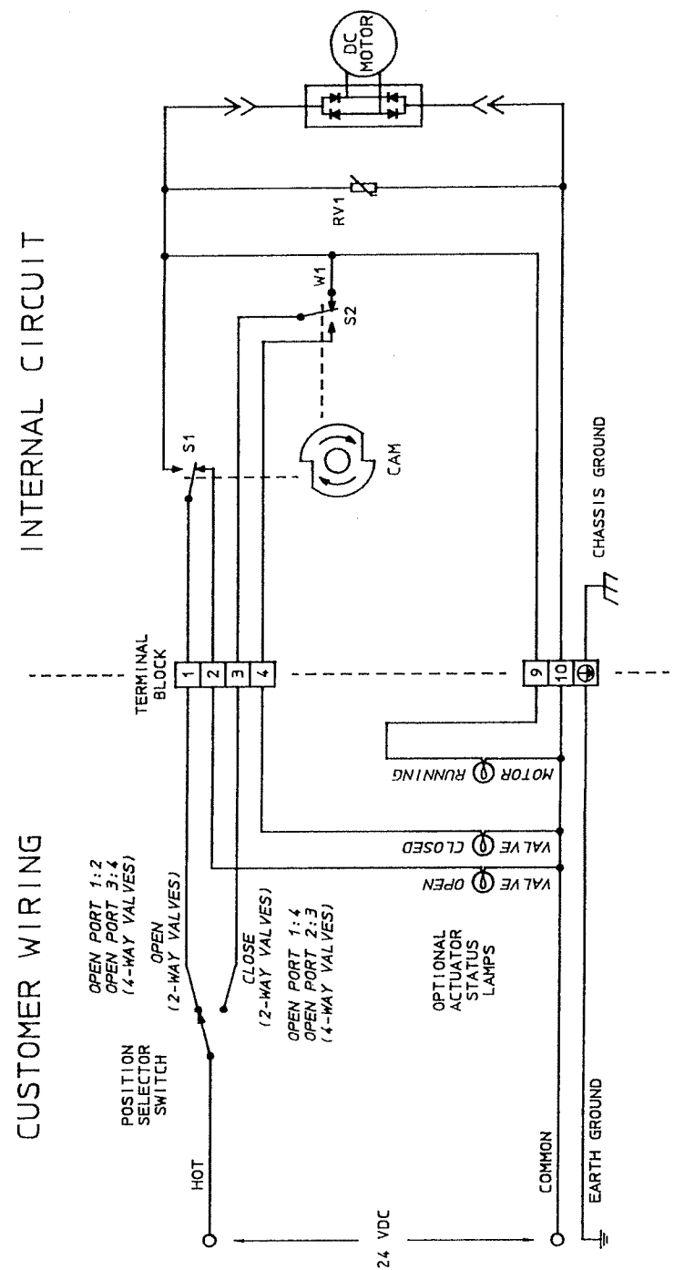
User Wiring and Internal Circuit
