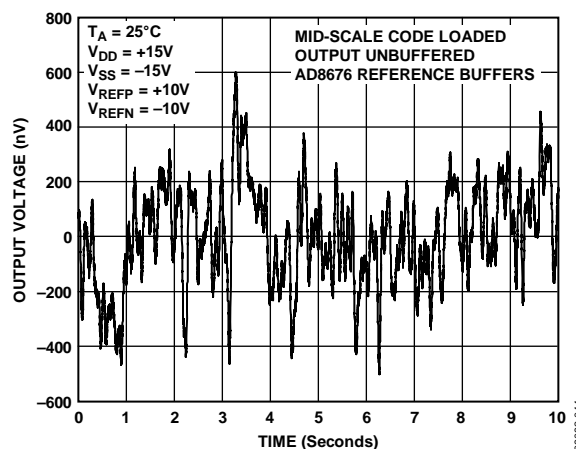
Figure 44. Voltage Output Noise, 0.1 Hz to 10 Hz Bandwidth
