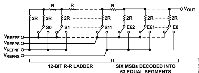
Figure 46. DAC Ladder Structure Serial Interface
