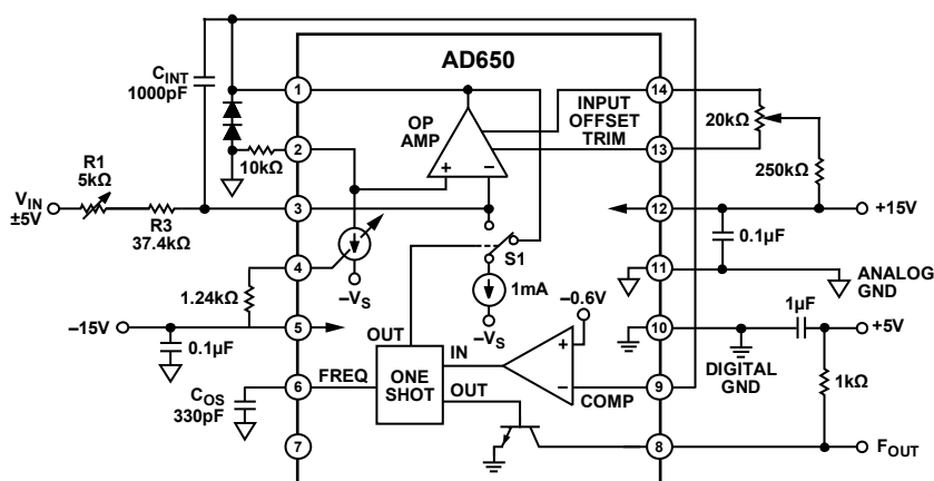
Figure 11. Connections for \pm 5 V Bipolar V/F with 0 kHz to 100 kHz TTL Output Rev. E | Page 10 of 20
